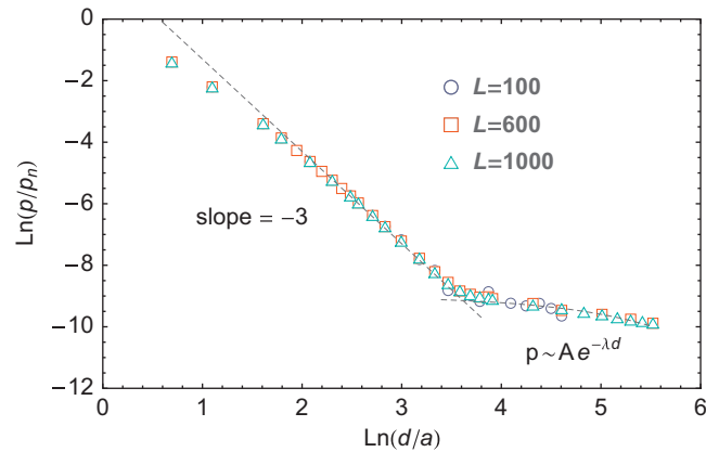
Fig. 5. Simulation results (symbols) of the p – d dependence at the longer range of d 's. The sizes of the membrane are shown in the labels. The other simulation parameters are k_B T = 10.0 , \kappa = 1.0 , and a = 1.0 . The scaling pressure is p_n = k_B T / a^3 .
