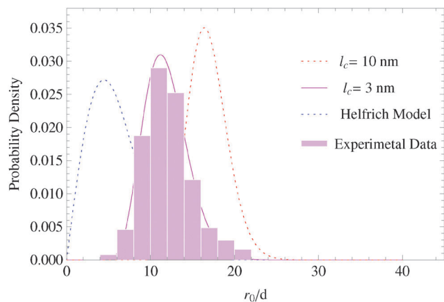
Fig. 4 Size distribution of vesicles with different values of l_c . In this figure, the horizontal axis is the normalized radius of the vesicle \xi = r_0/d and the vertical axis is the probability of finding vesicles within a certain radius. The dotted blue curve corresponds to the size distribution as predicted by linear curvature elasticity. 84 The solid magenta is obtained assuming l_c = 3 nm, which results in a shift in the size distribution, to larger sizes. Also the dotted red line corresponds to l_c = 10 nm which dramatically changes the cut-off radius as well as the mean radius of the vesicles. Based on the experimental data, 41 shown in the purple color, we have estimated the characteristic length for this kind of lauric acid vesicle to be about l_c = 3 nm. For our calculations, we have set \kappa_b = 20k_B T and d = 5 nm.
