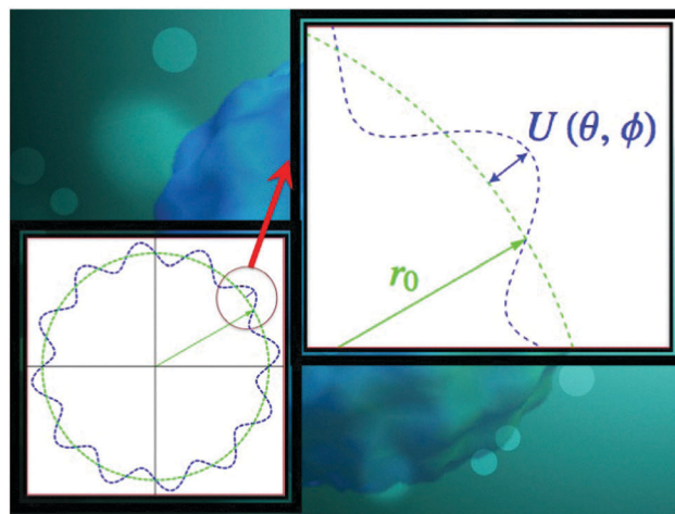
Fig. 2 Displacement field fluctuations of the surface of a spherical membrane. We have assumed that the fluctuations are normal to the surface. The fluctuating mid-plane displacement is normalized as u(\theta, \phi) = U(\theta, \phi)/r_0 .
