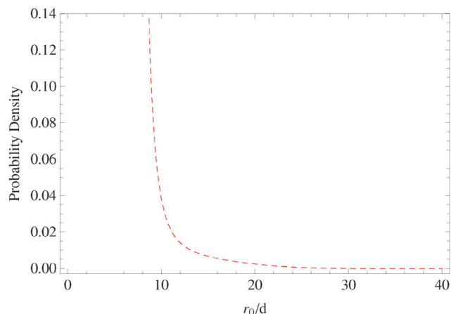
Fig. 5 Size distribution of vesicles with a negative fourth order modulus is shown qualitatively in this figure. In sharp contrast to experimental observations known so far, the distribution is discontinuous and is not a Gaussian distribution. Small-size vesicles are more probable not less. Finally, beyond a certain size, the vesicle becomes unstable. This plot is obtained by \ell_c = 2 nm. For larger values of \ell_c , the unstable region is shifted to larger sizes.
