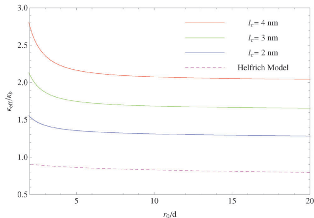
Fig. 3 Renormalized bending modulus for different values of \ell_c . Solid red, green and blue correspond to \ell_c = 4 nm, \ell_c = 3 nm and \ell_c = 2 nm, respectively. The dashed line is obtained from the Helfrich linear model in which \ell_c = 0 . The data have been calculated with \kappa_{\text{b}} = 20k_{\text{B}}T and d = 5 nm.
